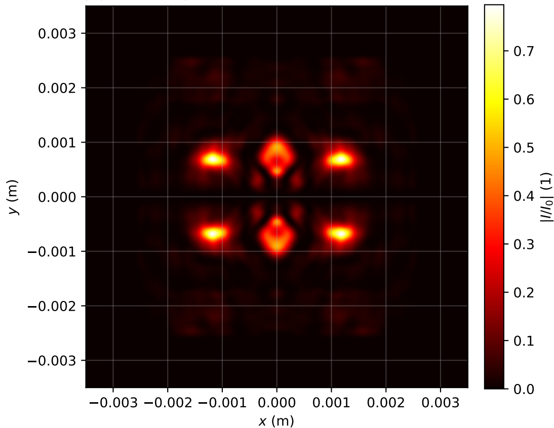
Intensity profile I(x, y, z = 1.990)/I_0 , P_{in}=17.0\text{Pcr} , artificial time
