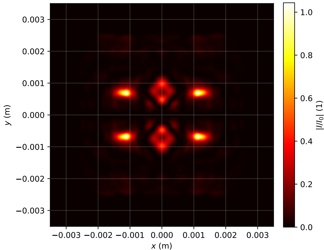
Intensity profile I(x, y, z = 2.070)/I_0 , P_{in}=17.0\text{Pcr} , artificial time
