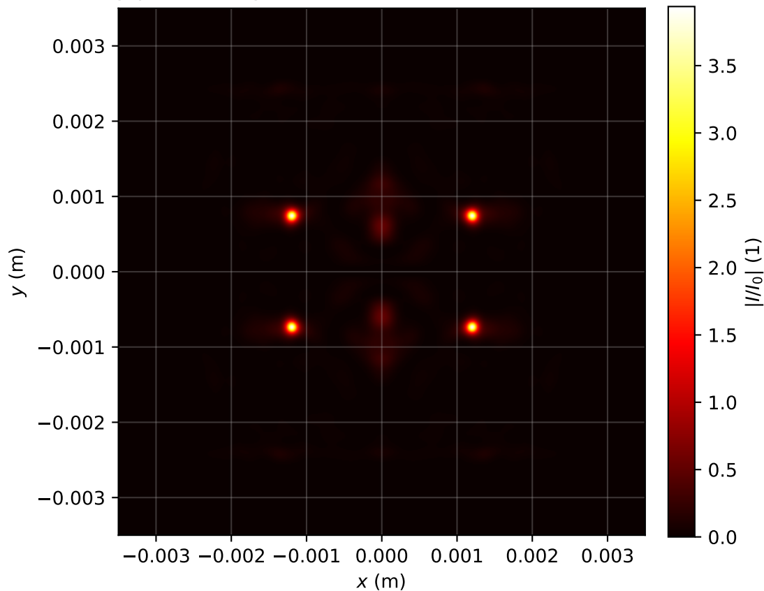
Intensity profile I(x, y, z = 2.309)/I_0 , P_{in}=17.0\text{Pcr} , artificial time
