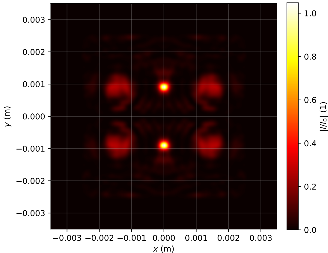
Intensity profile I(x, y, z = 2.866)/I_0 , P_{in}=17.0\text{Pcr} , artificial time
