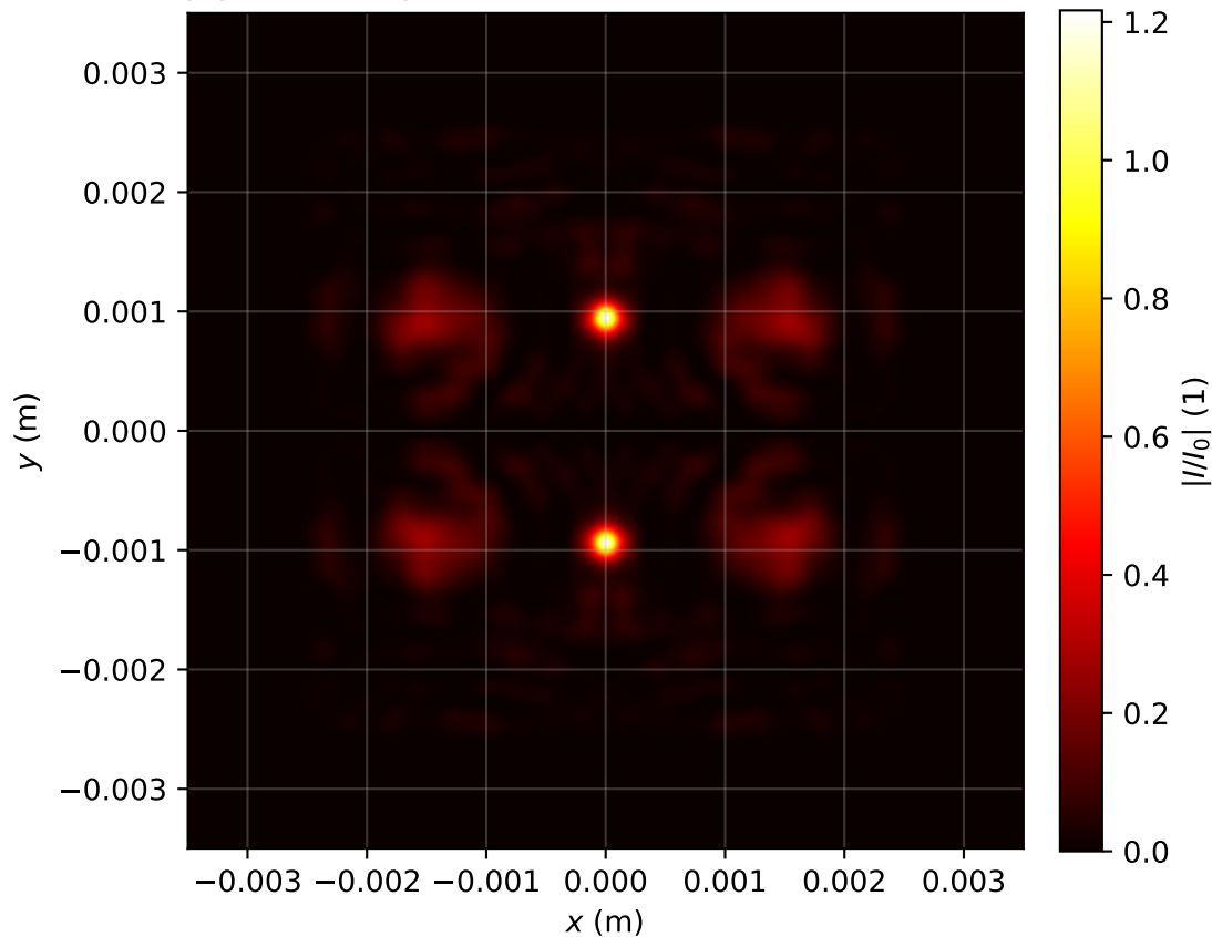
Intensity profile I(x, y, z = 2.946)/I_0 , P_{in}=17.0\text{Pcr} , artificial time
