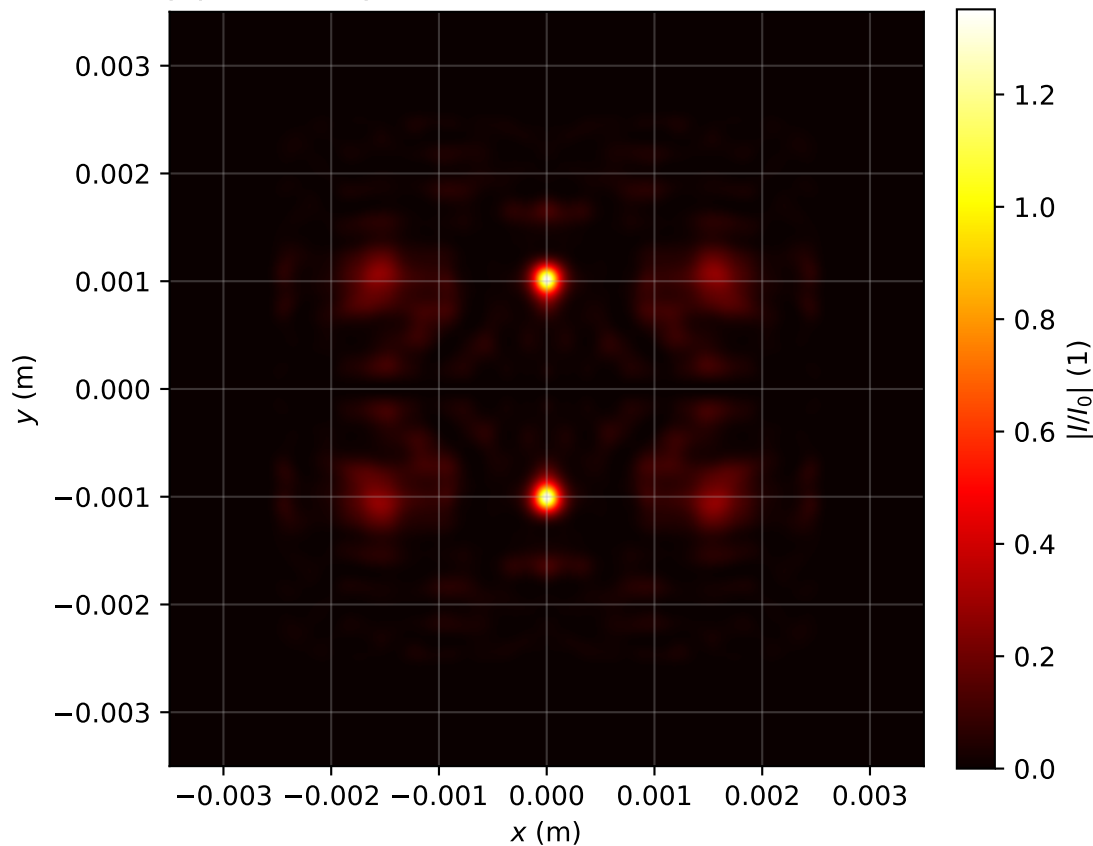
Intensity profile I(x, y, z = 3.105)/I_0 , P_{in}=17.0\text{Pcr} , artificial time
