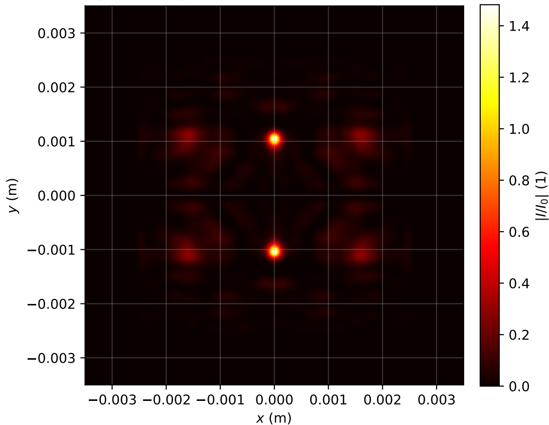
Intensity profile I(x, y, z = 3.184)/I_0 , P_{in}=17.0\text{Pcr} , artificial time
