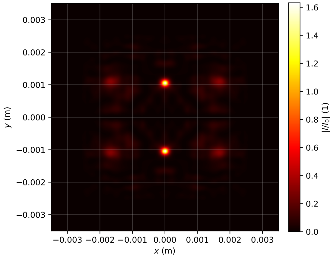
Intensity profile I(x, y, z = 3.264)/I_0 , P_{in}=17.0\text{Pcr} , artificial time
