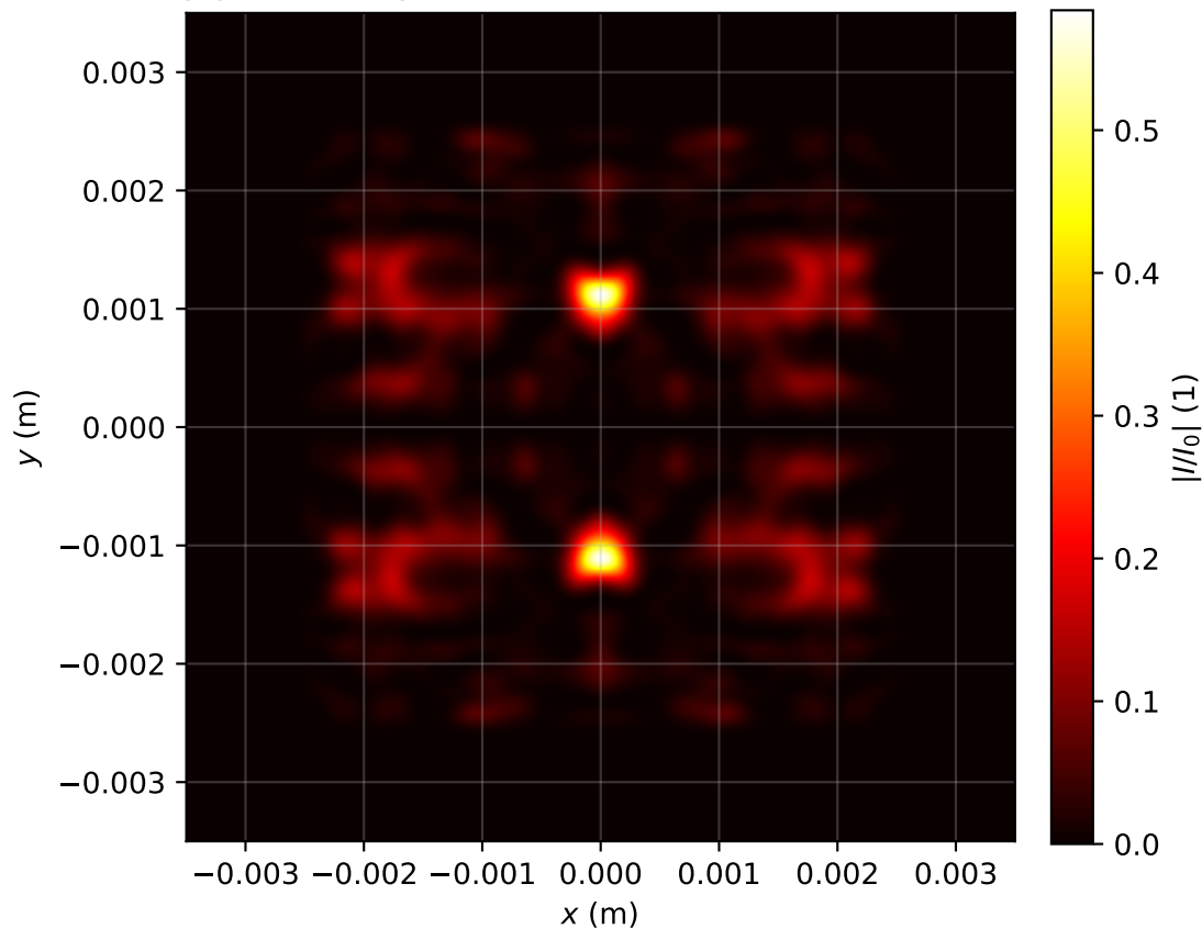
Intensity profile I(x, y, z = 3.582)/I_0 , P_{in}=17.0\text{Pcr} , artificial time
