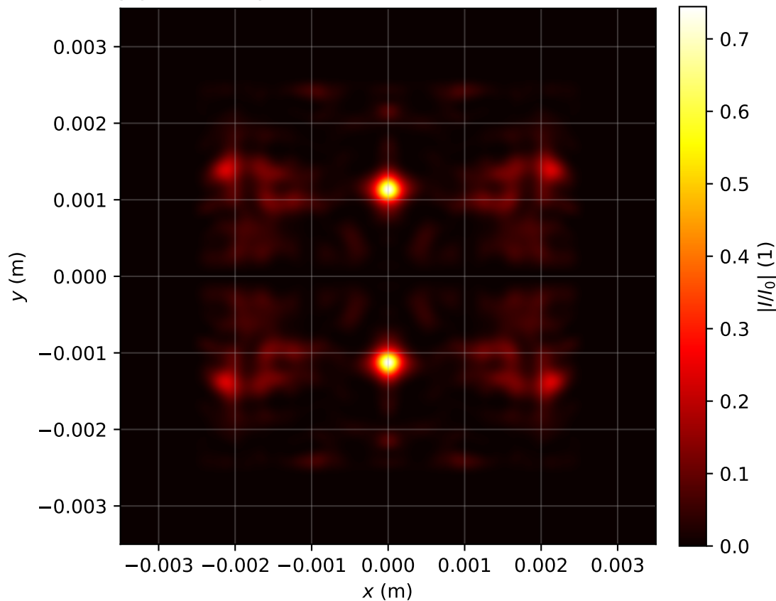
Intensity profile I(x, y, z = 3.821)/I_0 , P_{in}=17.0P_{cr} , artificial time
