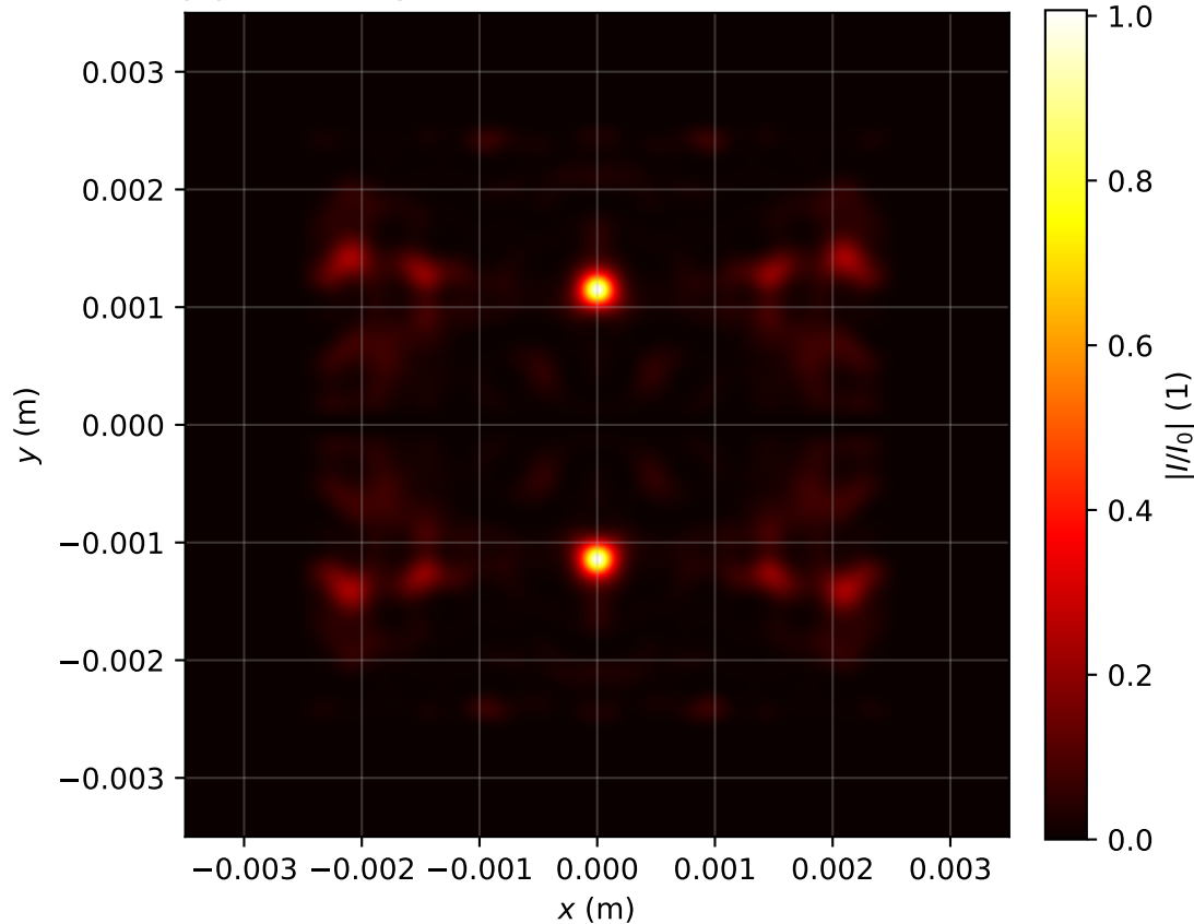
Intensity profile I(x, y, z = 3.981)/I_0 , P_{in}=17.0\text{Pcr} , artificial time
