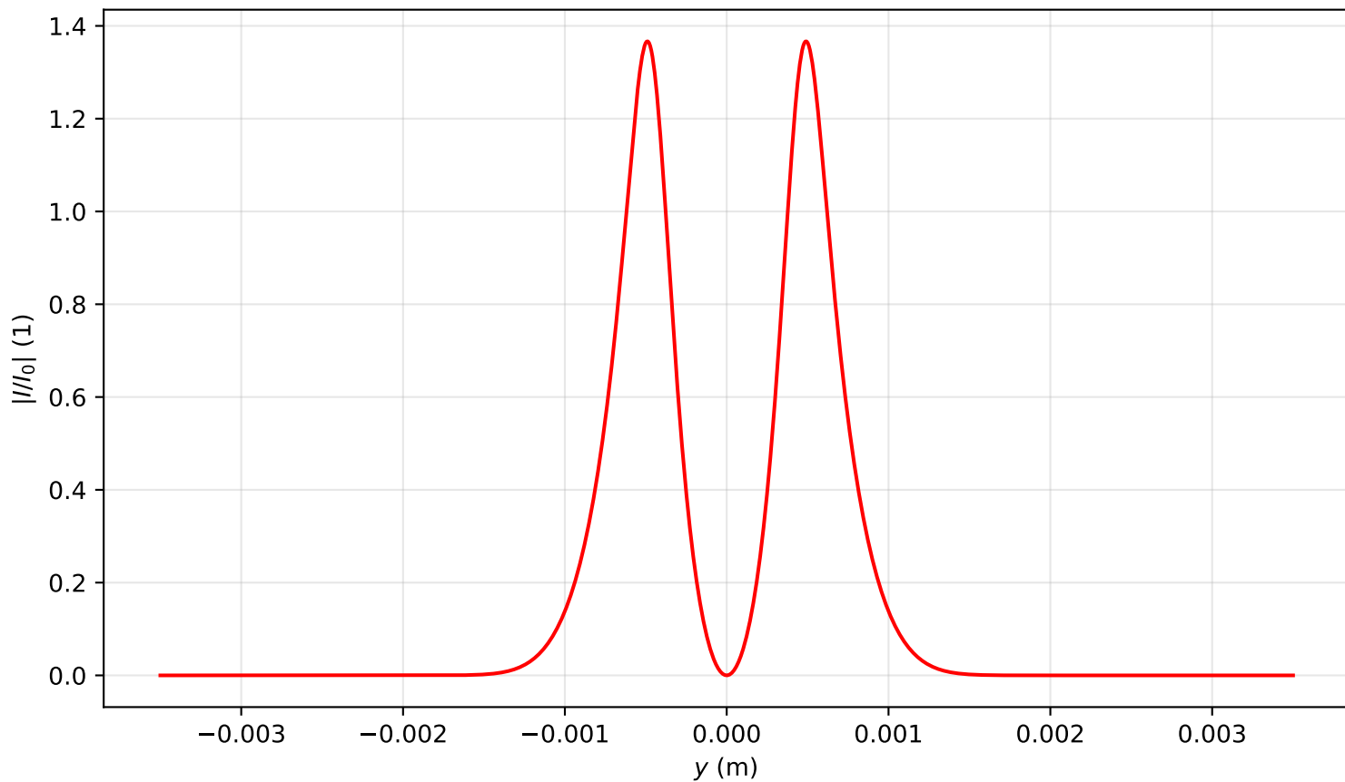
Intensity profile I(x=0, y, z=0.159)/I_0 , P_{in}=17.0P_{cr} , artificial time
