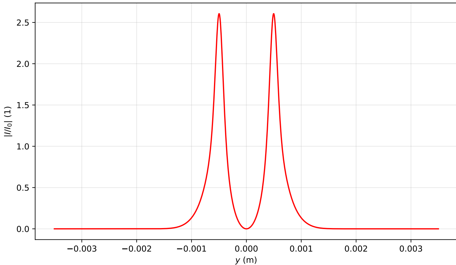
Intensity profile I(x=0, y, z=0.239)/I_0 , P_{in}=17.0P_{cr} , artificial time
