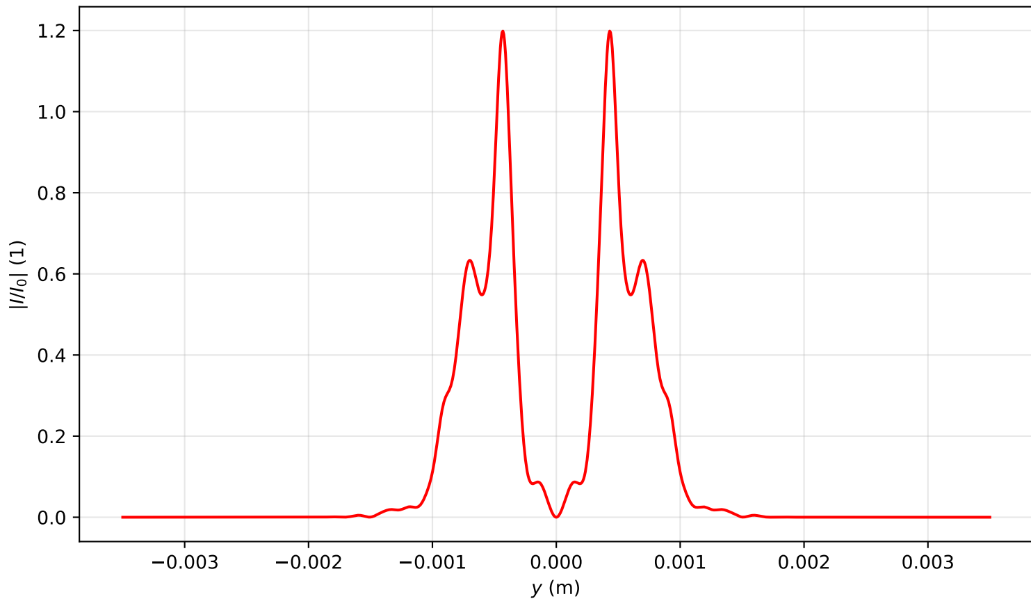
Intensity profile I(x=0, y, z=0.557)/I_0 , P_{in}=17.0P_{cr} , artificial time
