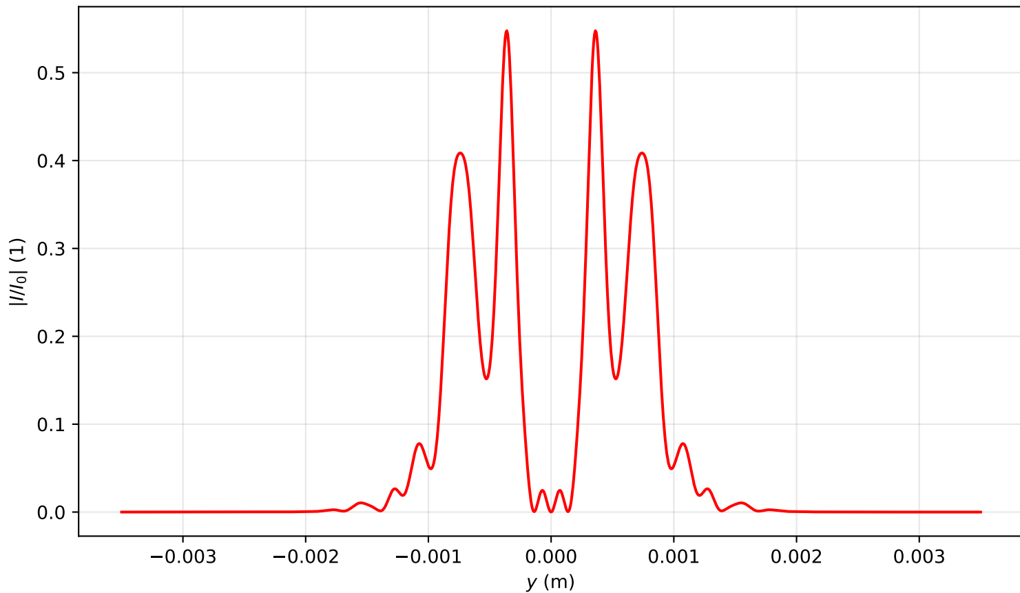
Intensity profile I(x=0, y, z=0.637)/I_0 , P_{in}=17.0P_{cr} , artificial time
