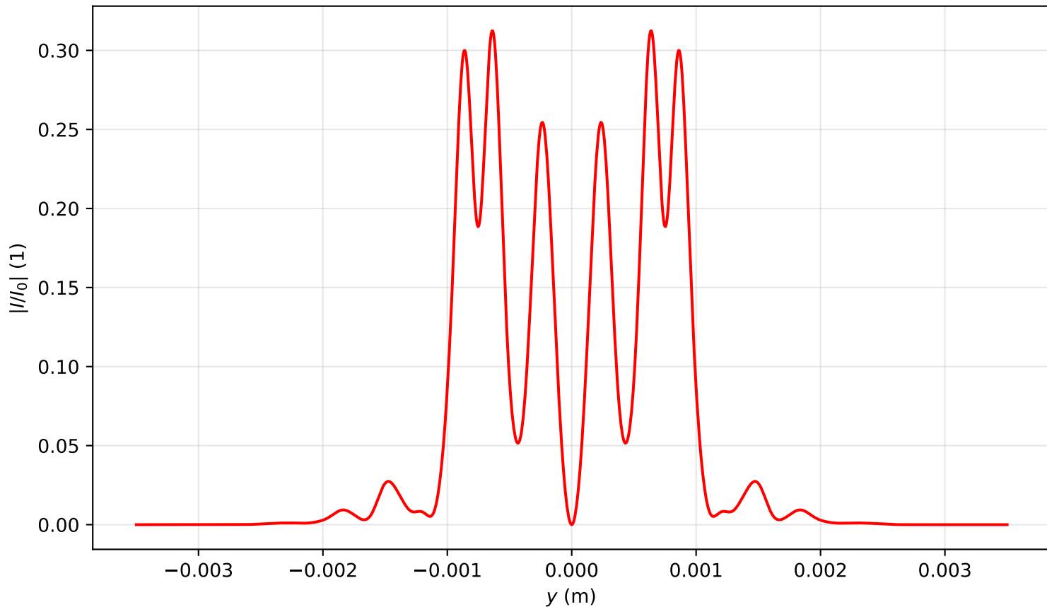
Intensity profile I(x=0, y, z=0.796)/I_0 , P_{in}=17.0P_{cr} , artificial time
