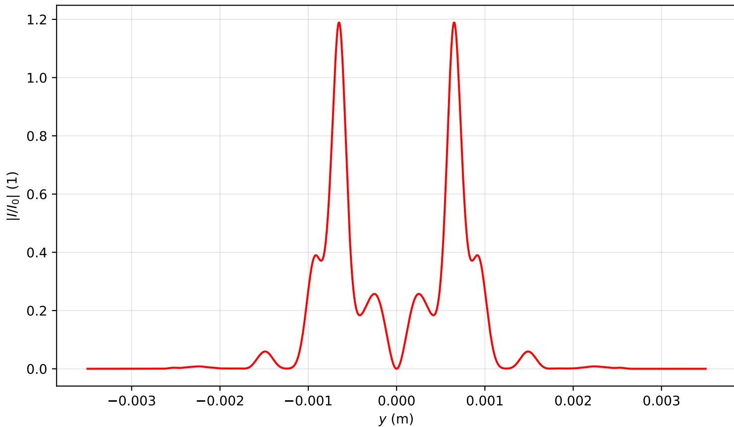
Intensity profile I(x=0, y, z=1.035)/I_0 , P_{in}=17.0P_{cr} , artificial time
