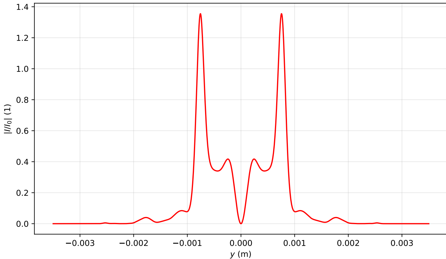
Intensity profile I(x=0, y, z=1.194)/I_0 , P_{in}=17.0\text{Pcr} , artificial time
