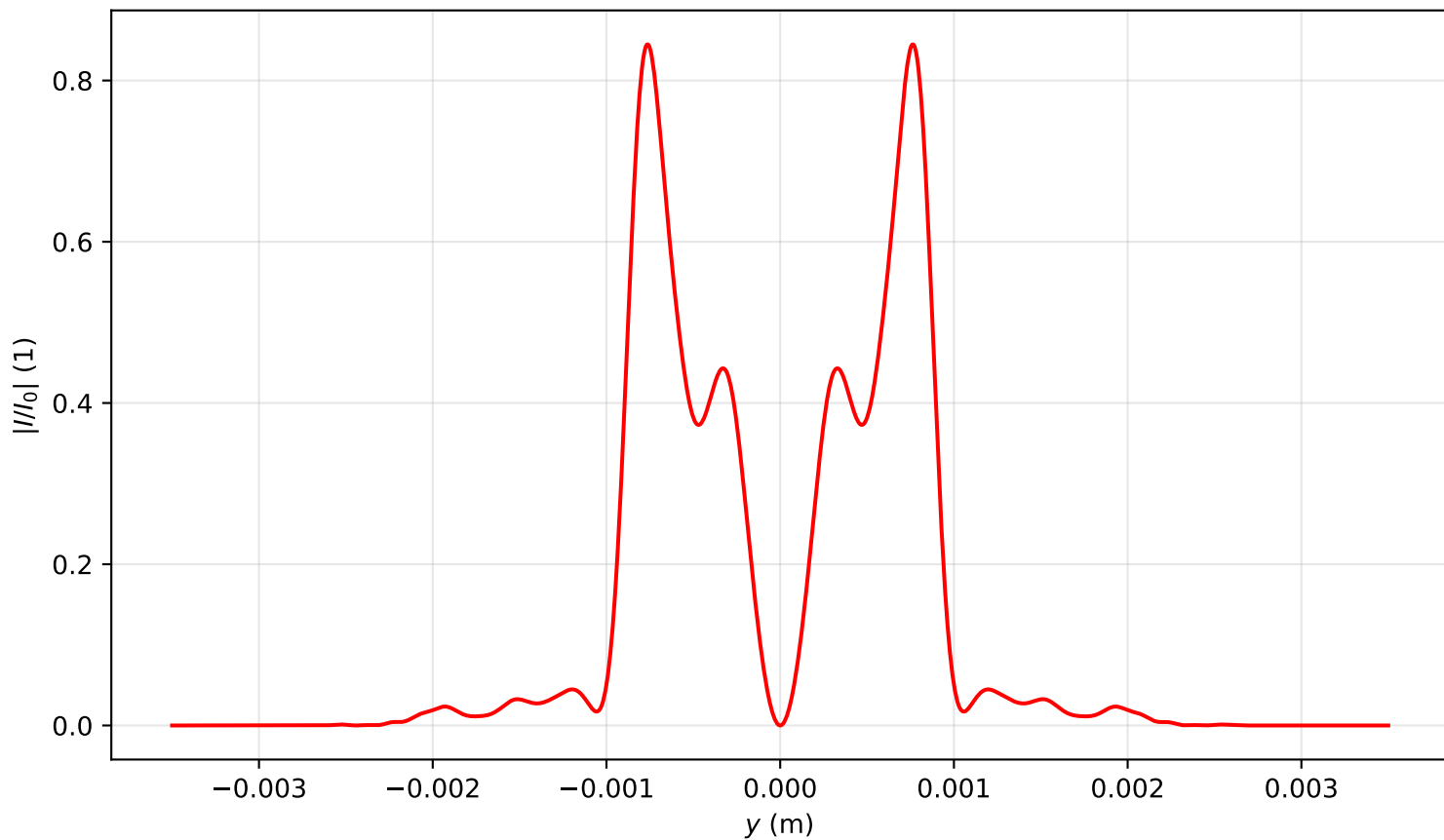
Intensity profile I(x=0, y, z=1.274)/I_0 , Pin=17.0Pcr, artificial time
