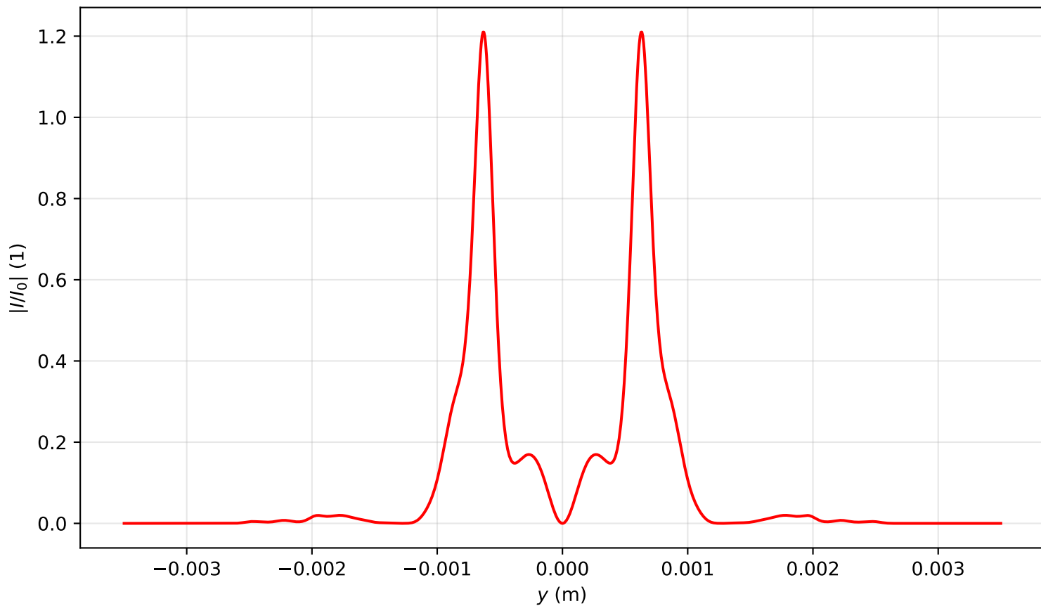
Intensity profile I(x=0, y, z=1.433)/I_0 , P_{in}=17.0P_{cr} , artificial time
