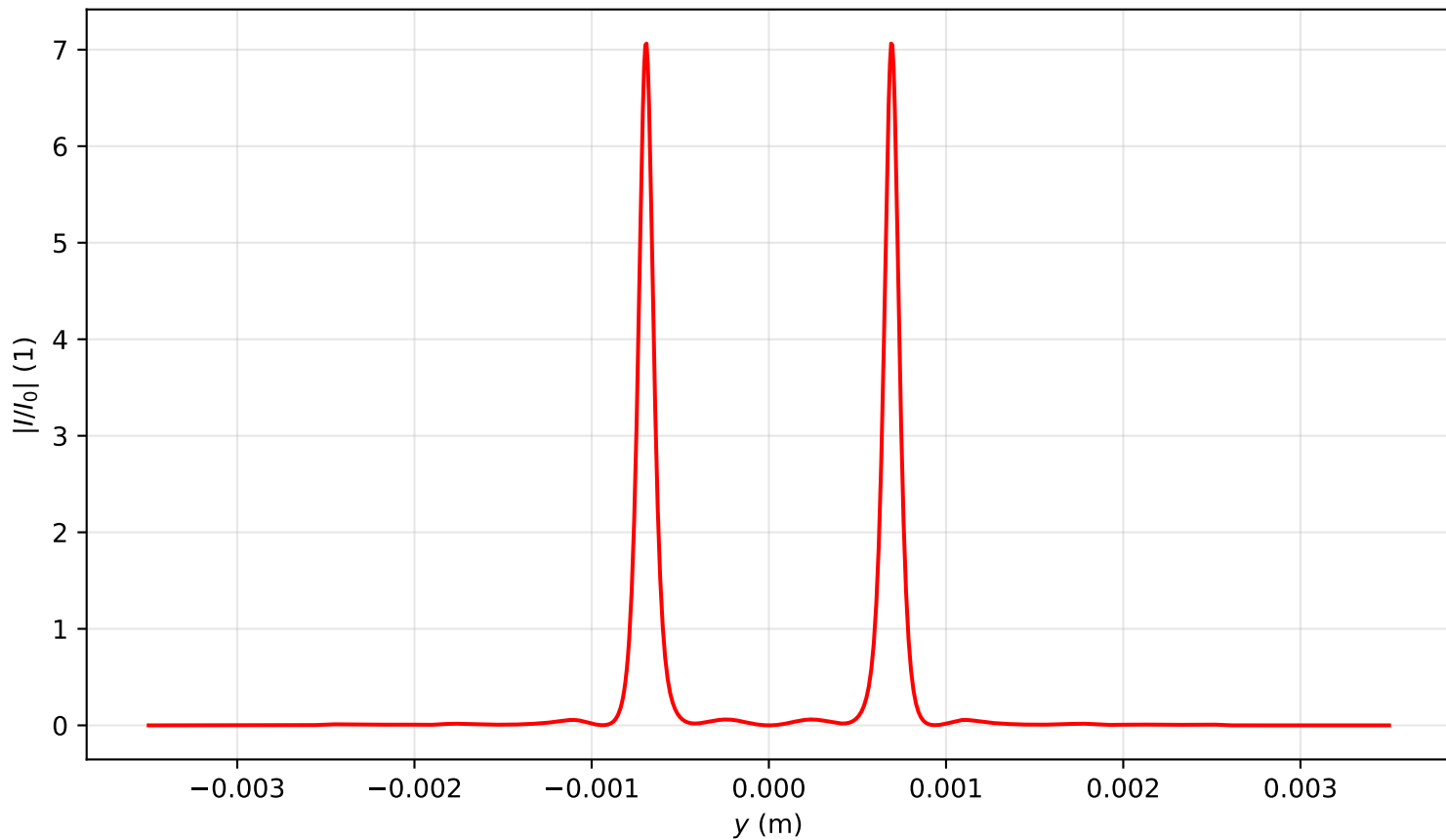
Intensity profile I(x=0, y, z=1.672)/I_0 , \text{Pin}=17.0\text{Pcr} , artificial time
