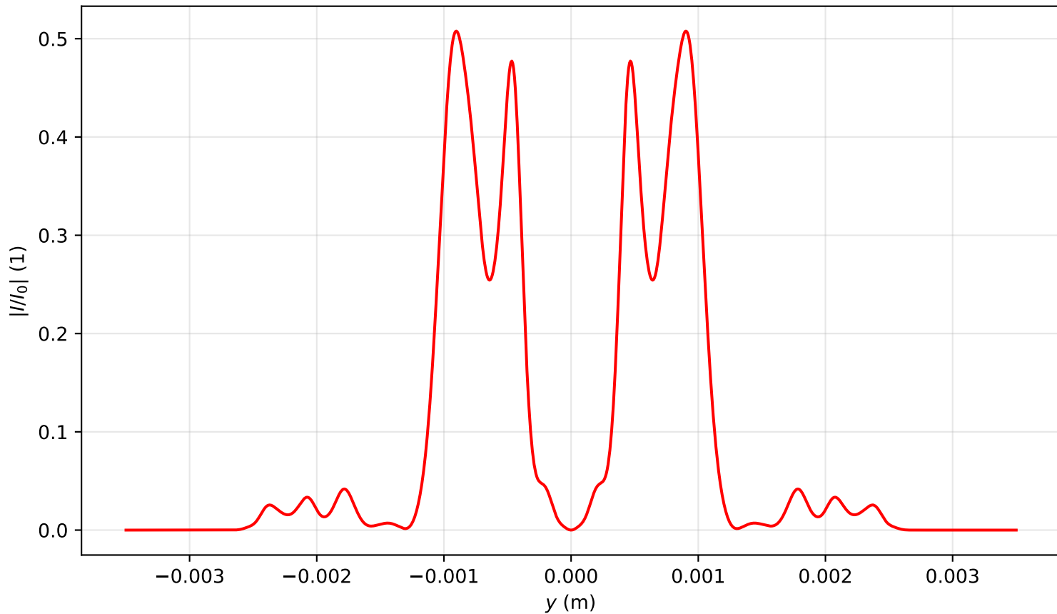
Intensity profile I(x=0, y, z=1.990)/I_0 , P_{in}=17.0P_{cr} , artificial time
