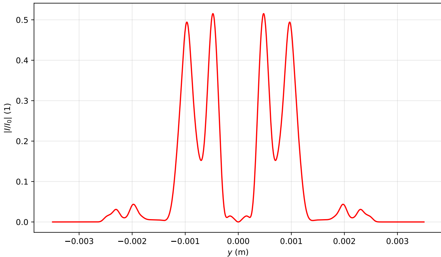
Intensity profile I(x=0, y, z=2.070)/I_0 , P_{in}=17.0\text{Pcr} , artificial time
