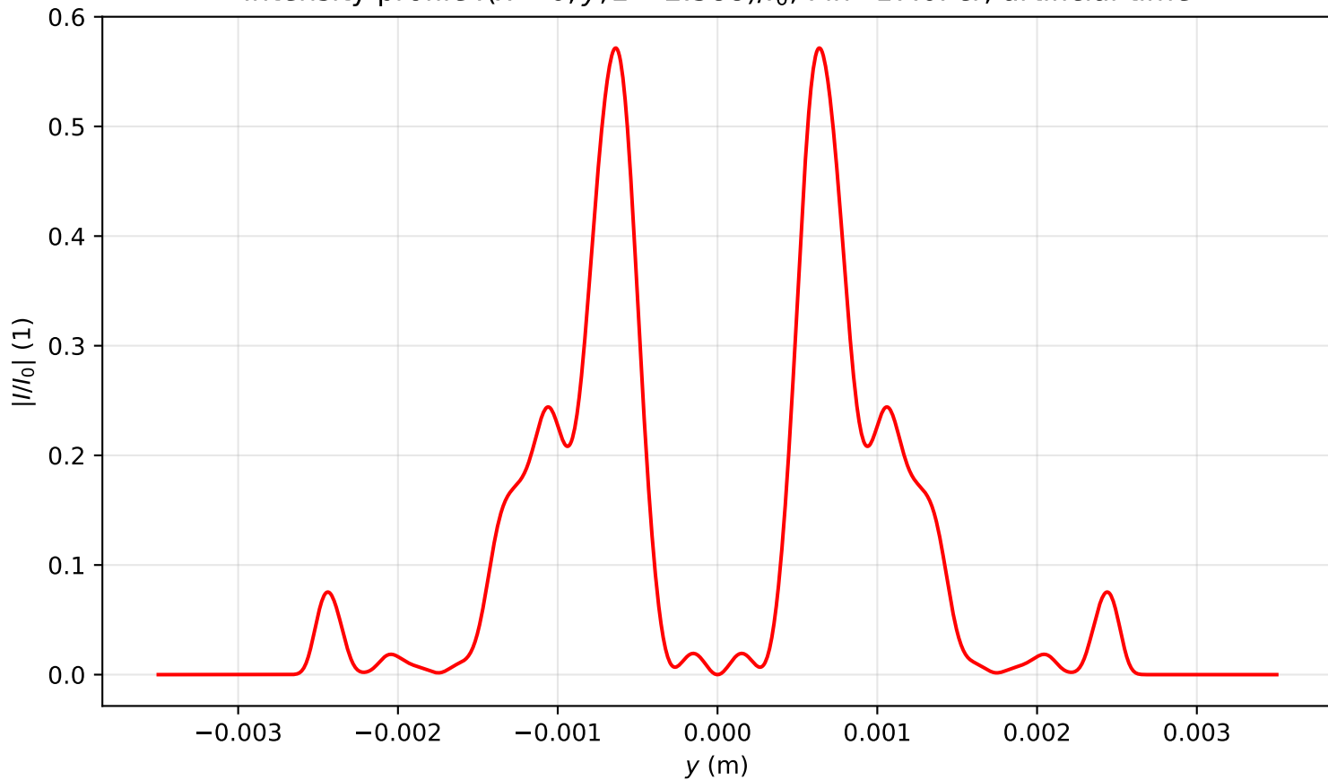
Intensity profile I(x=0, y, z=2.388)/I_0 , P_{in}=17.0P_{cr} , artificial time
