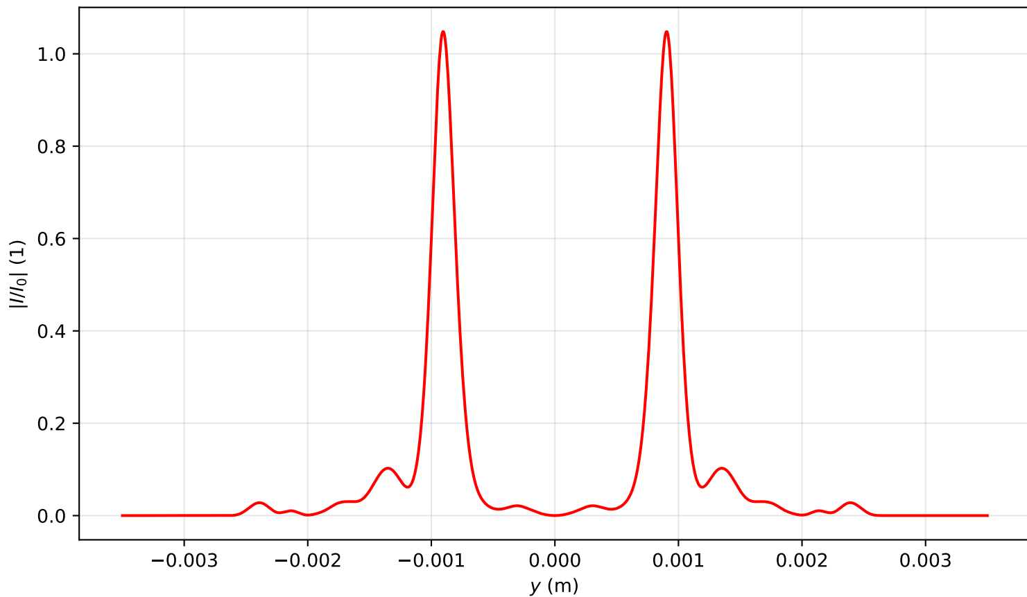
Intensity profile I(x=0, y, z=2.866)/I_0 , P_{in}=17.0P_{cr} , artificial time
