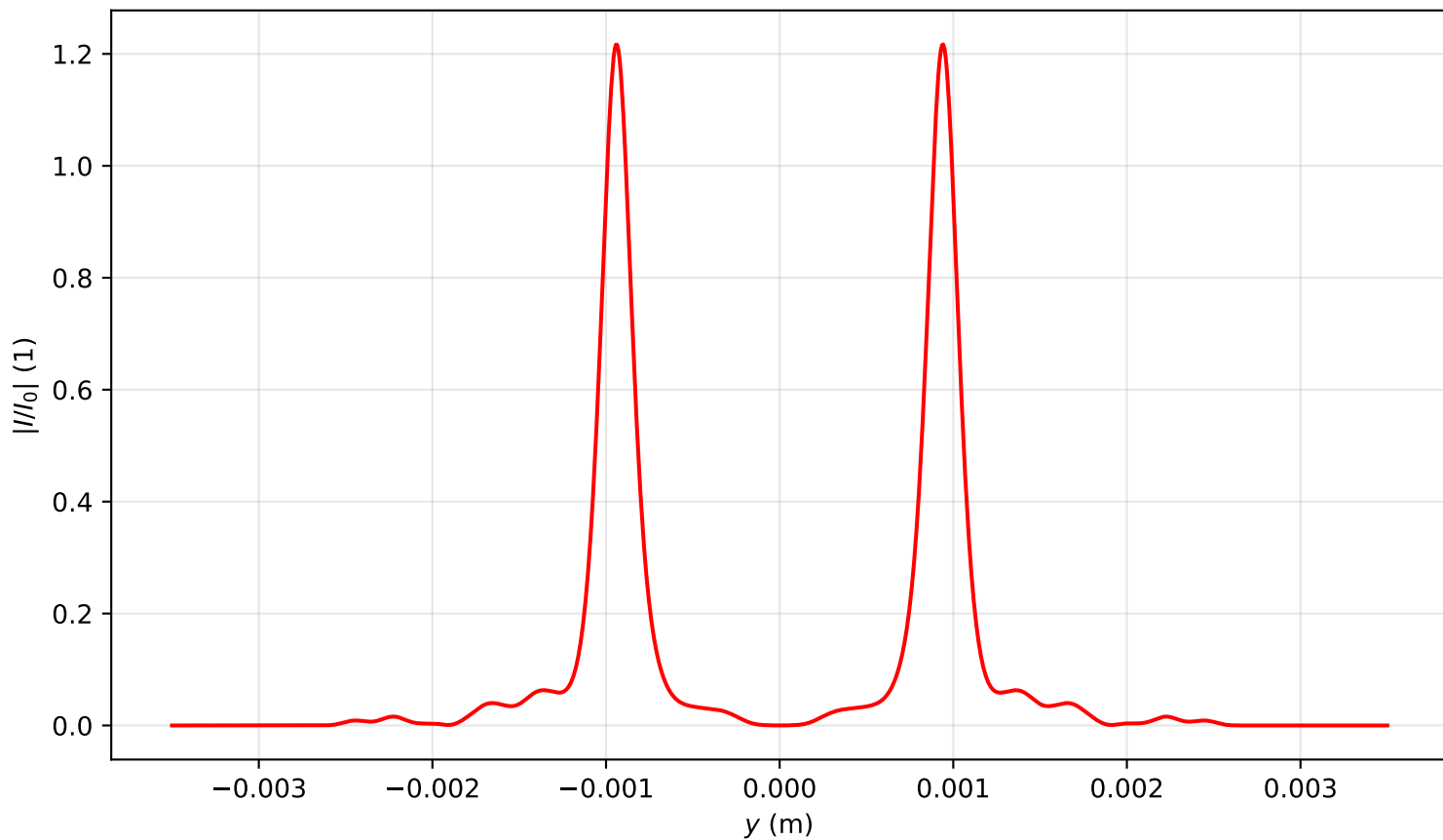
Intensity profile I(x=0, y, z=2.946)/I_0 , P_{in}=17.0P_{cr} , artificial time
