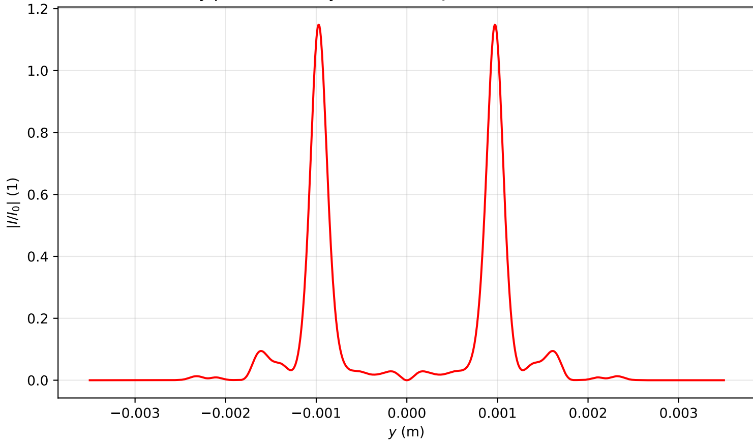
Intensity profile I(x=0, y, z=3.025)/I_0 , P_{in}=17.0P_{cr} , artificial time
