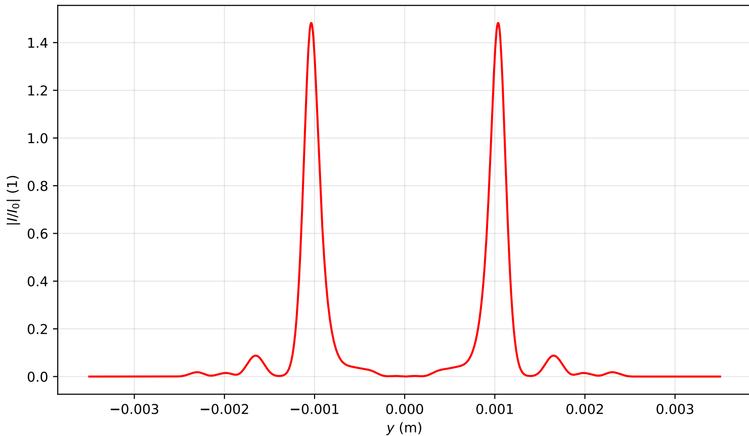
Intensity profile I(x=0, y, z=3.184)/I_0 , P_{in}=17.0\text{Pcr} , artificial time
