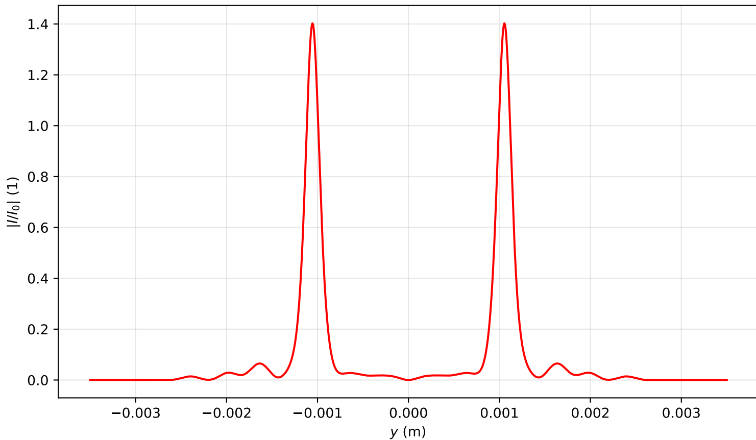
Intensity profile I(x=0, y, z=3.344)/I_0 , P_{in}=17.0\text{Pcr} , artificial time
