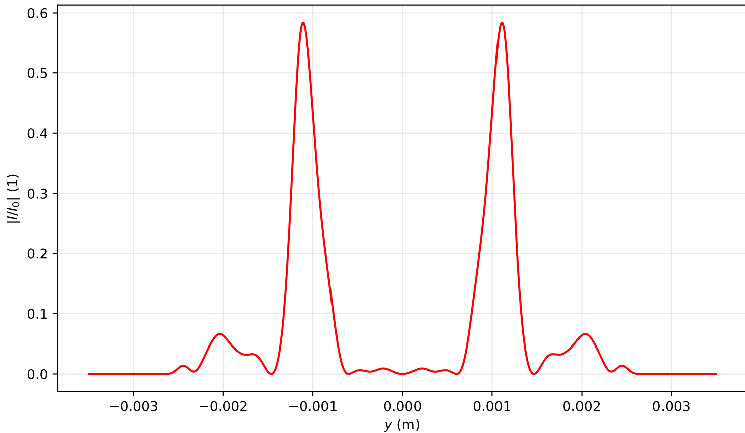
Intensity profile I(x=0, y, z=3.582)/I_0 , P_{in}=17.0\text{Pcr} , artificial time
