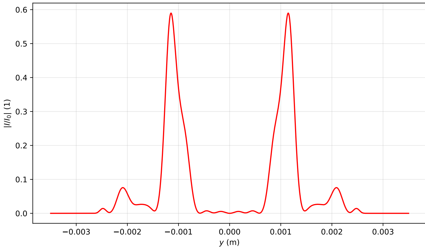
Intensity profile I(x=0, y, z=3.662)/I_0 , P_{in}=17.0\text{Pcr} , artificial time
