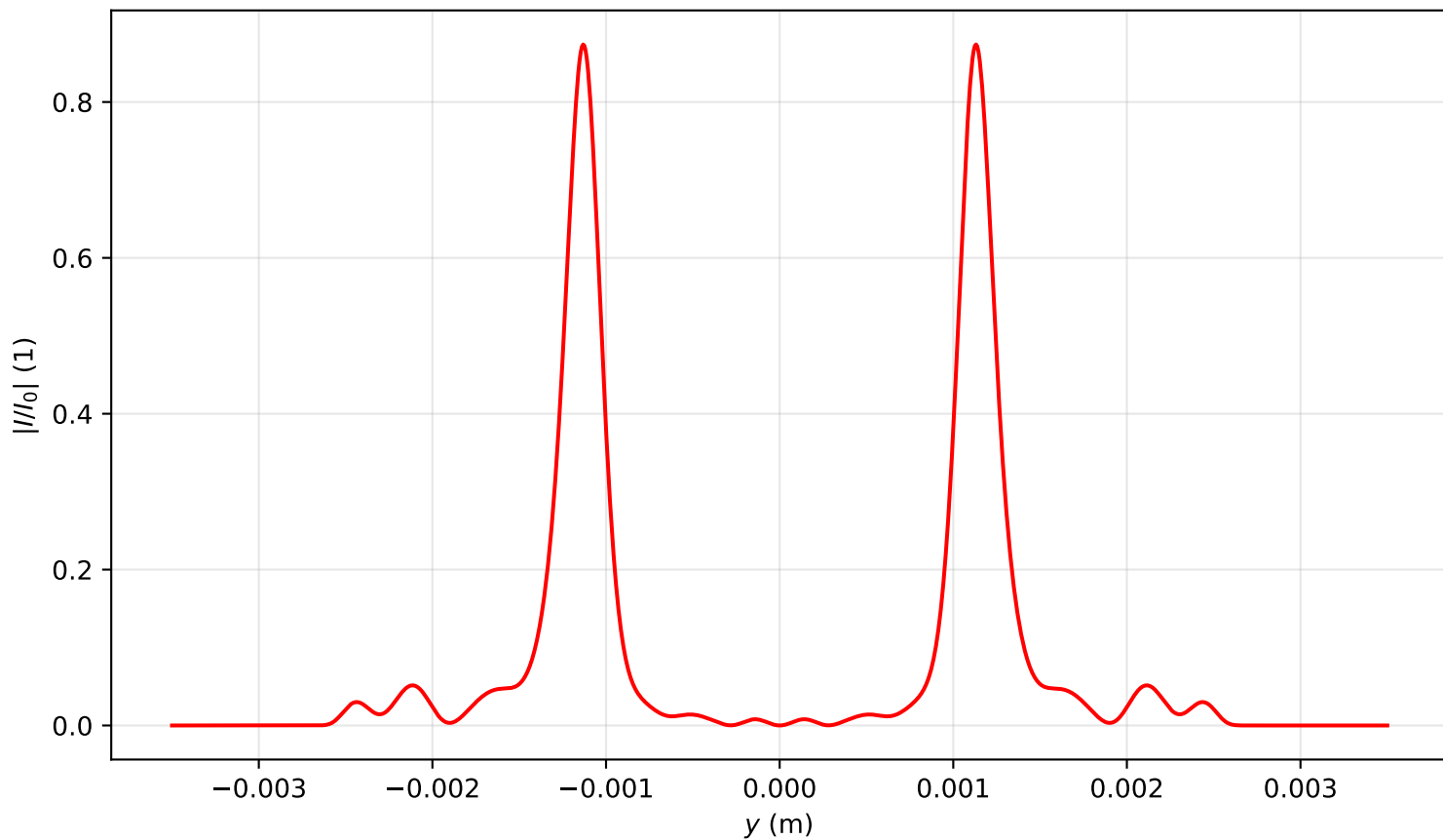
Intensity profile I(x=0, y, z=3.901)/I_0 , P_{in}=17.0\text{Pcr} , artificial time
