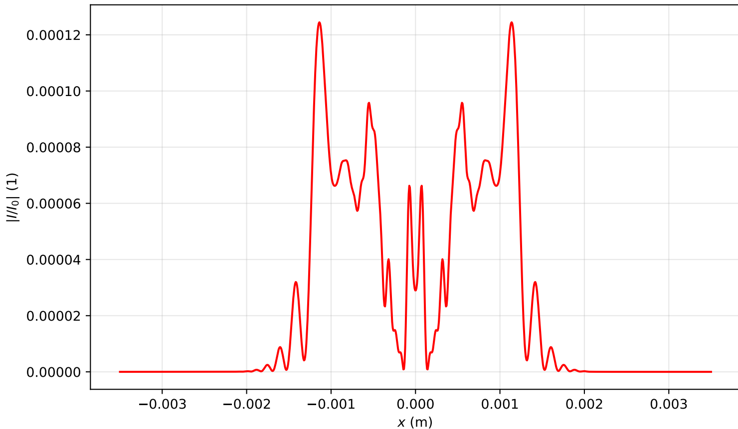
Intensity profile I(x, y = 0, z = 0.398)/I_0 , P_{in}=18.0P_{cr} , artificial time
