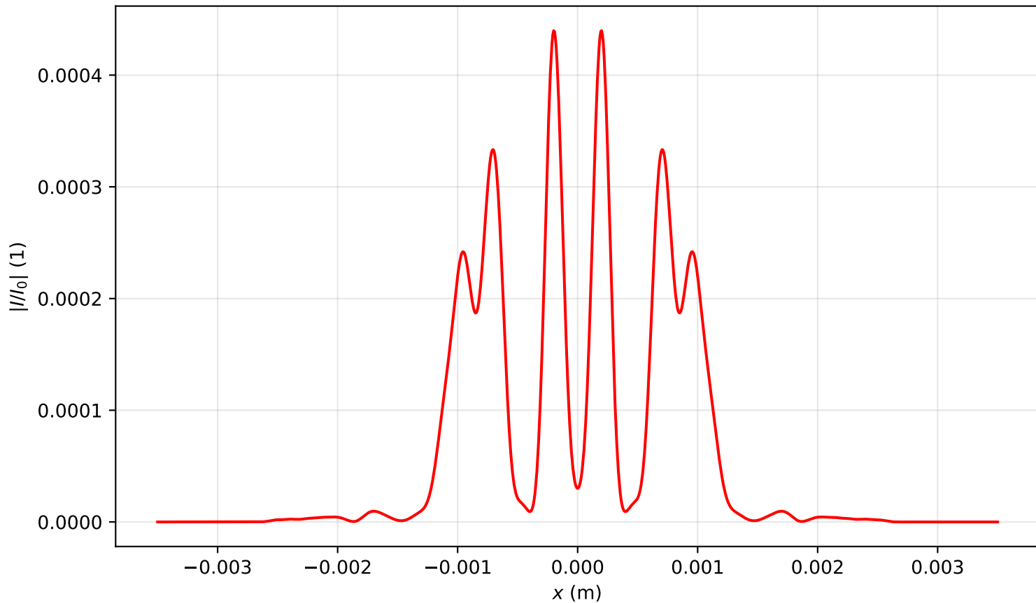
Intensity profile I(x, y = 0, z = 0.876)/I_0 , P_{in}=18.0P_{cr} , artificial time
