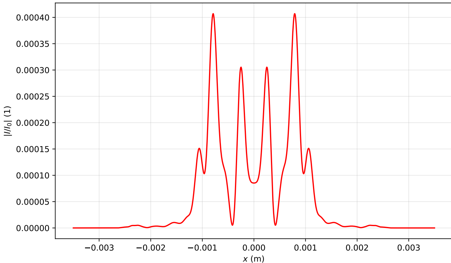
Intensity profile I(x, y = 0, z = 0.955)/I_0 , P_{in}=18.0\text{Pcr} , artificial time
