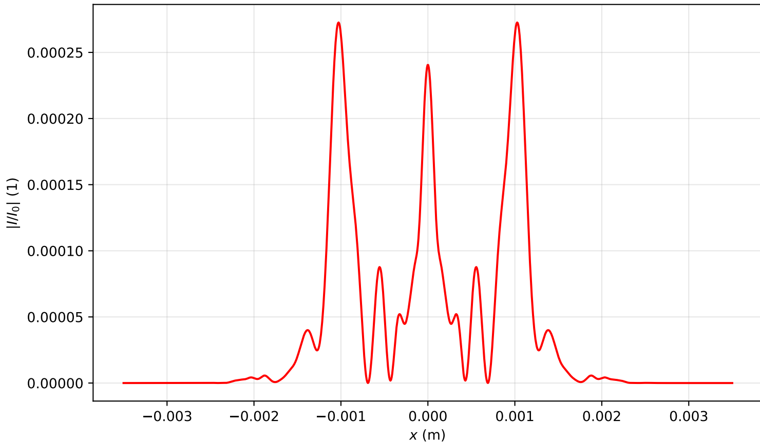
Intensity profile I(x, y = 0, z = 1.115)/I_0 , P_{in}=18.0P_{cr} , artificial time
