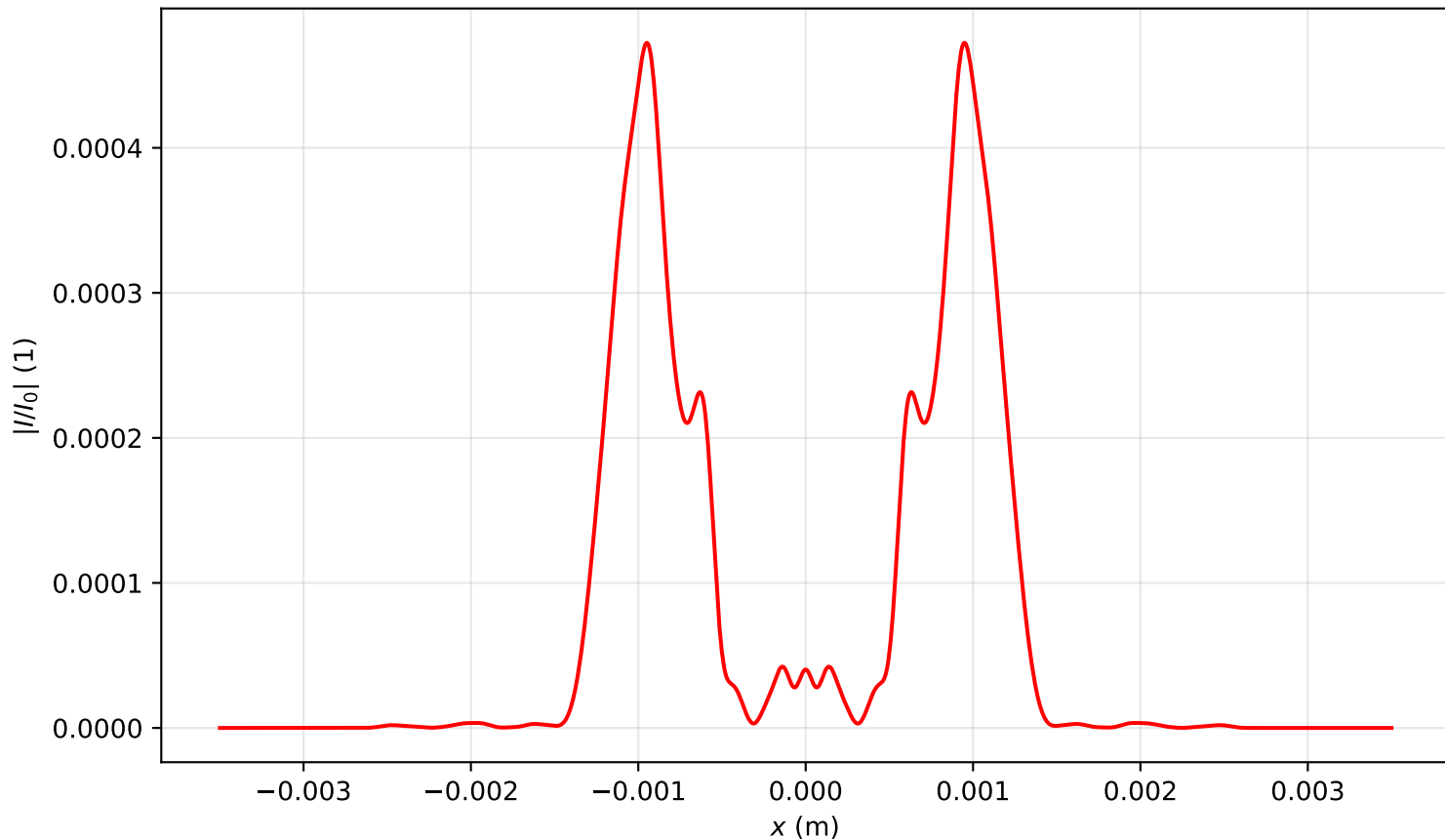
Intensity profile I(x, y = 0, z = 1.353)/I_0 , \text{Pin}=18.0\text{Pcr} , artificial time
