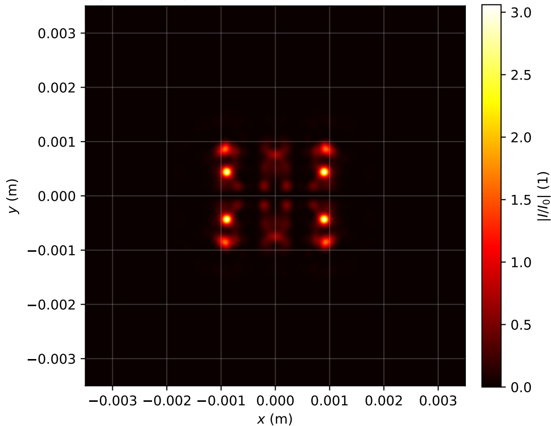
Intensity profile I(x, y, z = 0.876)/I_0 , P_{in}=18.0\text{Pcr} , artificial time
