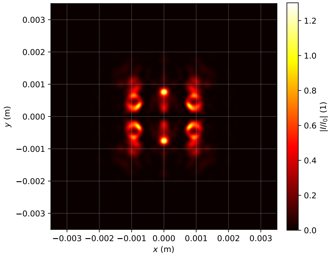
Intensity profile I(x, y, z = 1.194)/I_0 , P_{in}=18.0\text{Pcr} , artificial time
