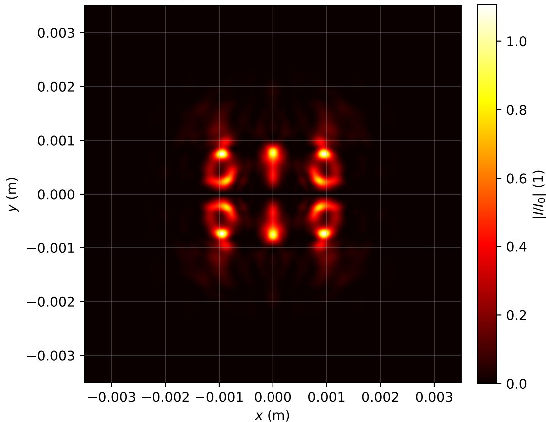
Intensity profile I(x, y, z = 1.274)/I_0 , P_{in}=18.0\text{Pcr} , artificial time
