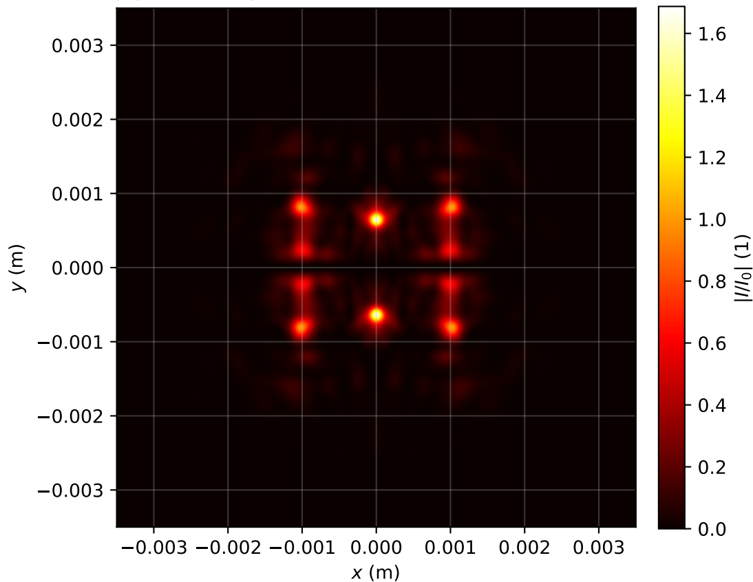
Intensity profile I(x, y, z = 1.433)/I_0 , P_{in}=18.0\text{Pcr} , artificial time
