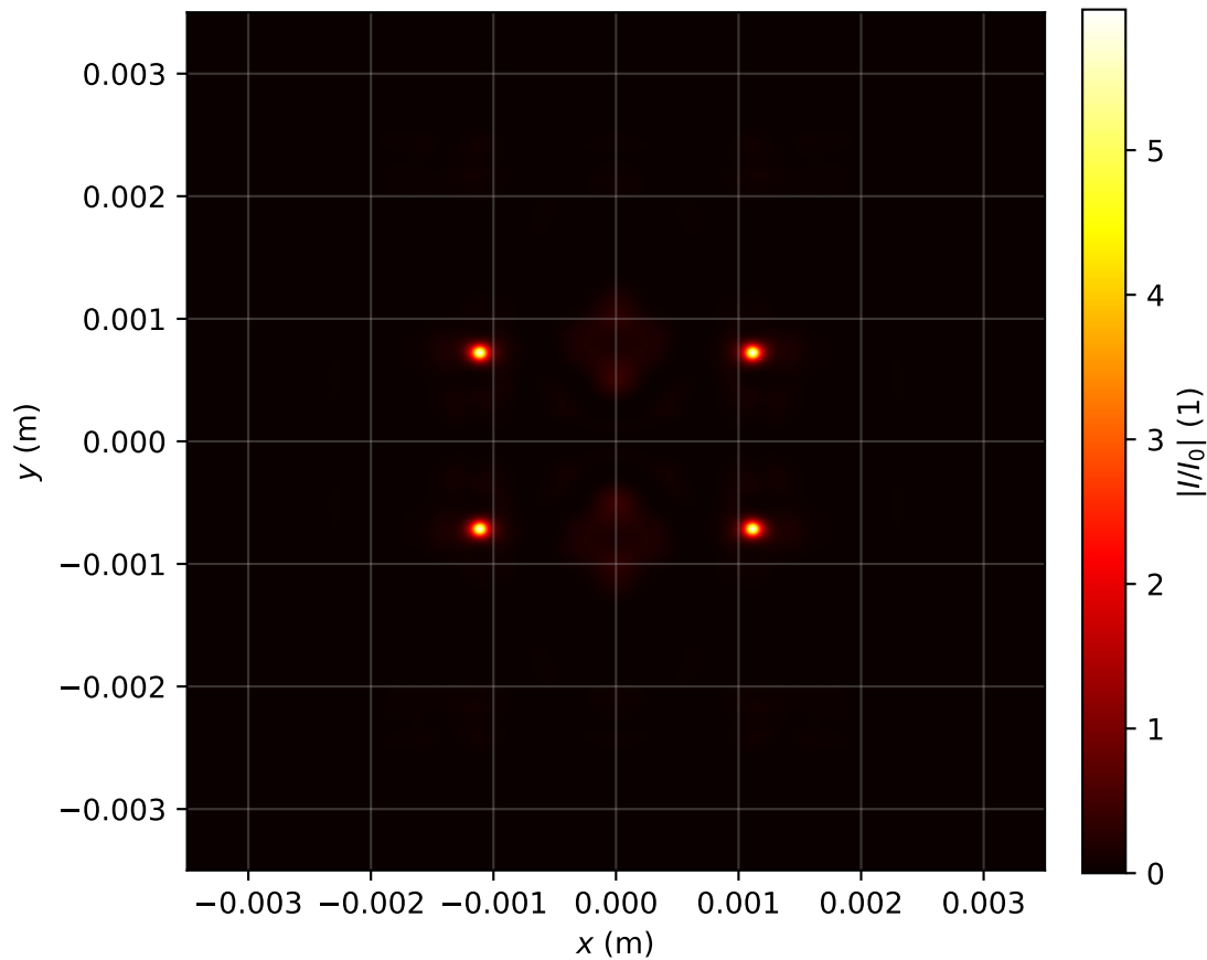
Intensity profile I(x, y, z = 2.070)/I_0 , P_{in}=18.0\text{Pcr} , artificial time
