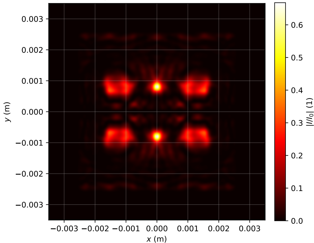
Intensity profile I(x, y, z = 2.548)/I_0 , P_{in}=18.0\text{Pcr} , artificial time
