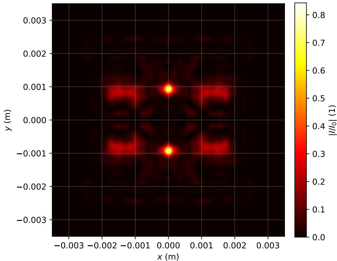
Intensity profile I(x, y, z = 2.786)/I_0 , P_{in}=18.0\text{Pcr} , artificial time
