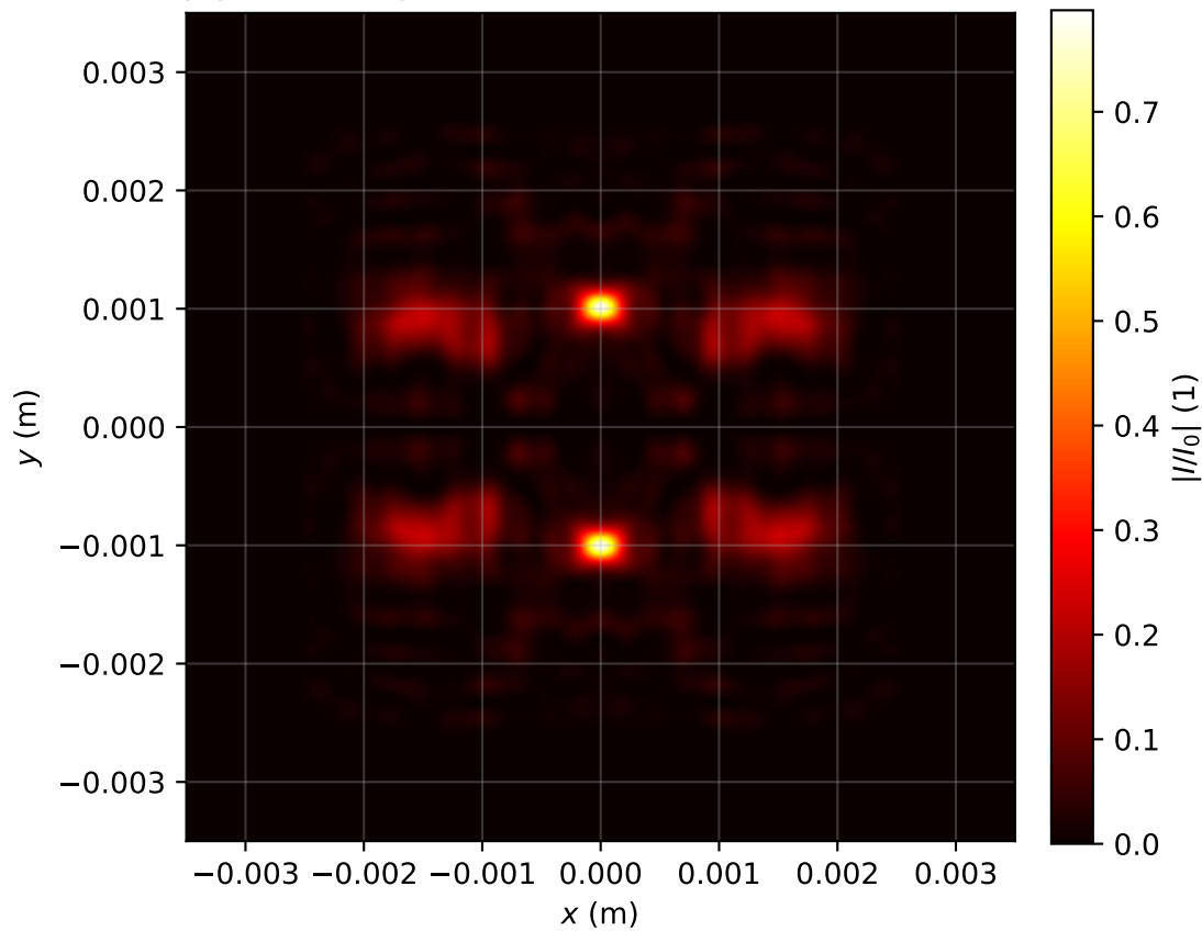
Intensity profile I(x, y, z = 2.946)/I_0 , P_{in}=18.0\text{Pcr} , artificial time
