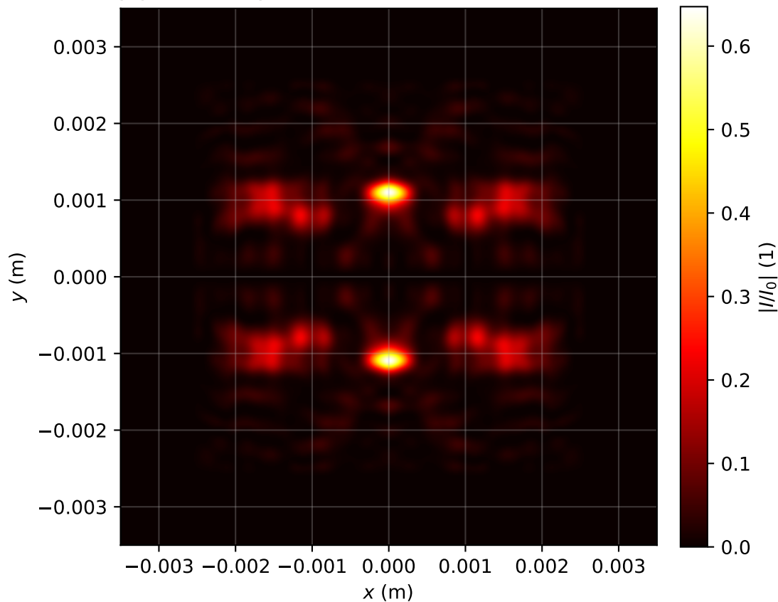
Intensity profile I(x, y, z = 3.105)/I_0 , P_{in}=18.0\text{Pcr} , artificial time
