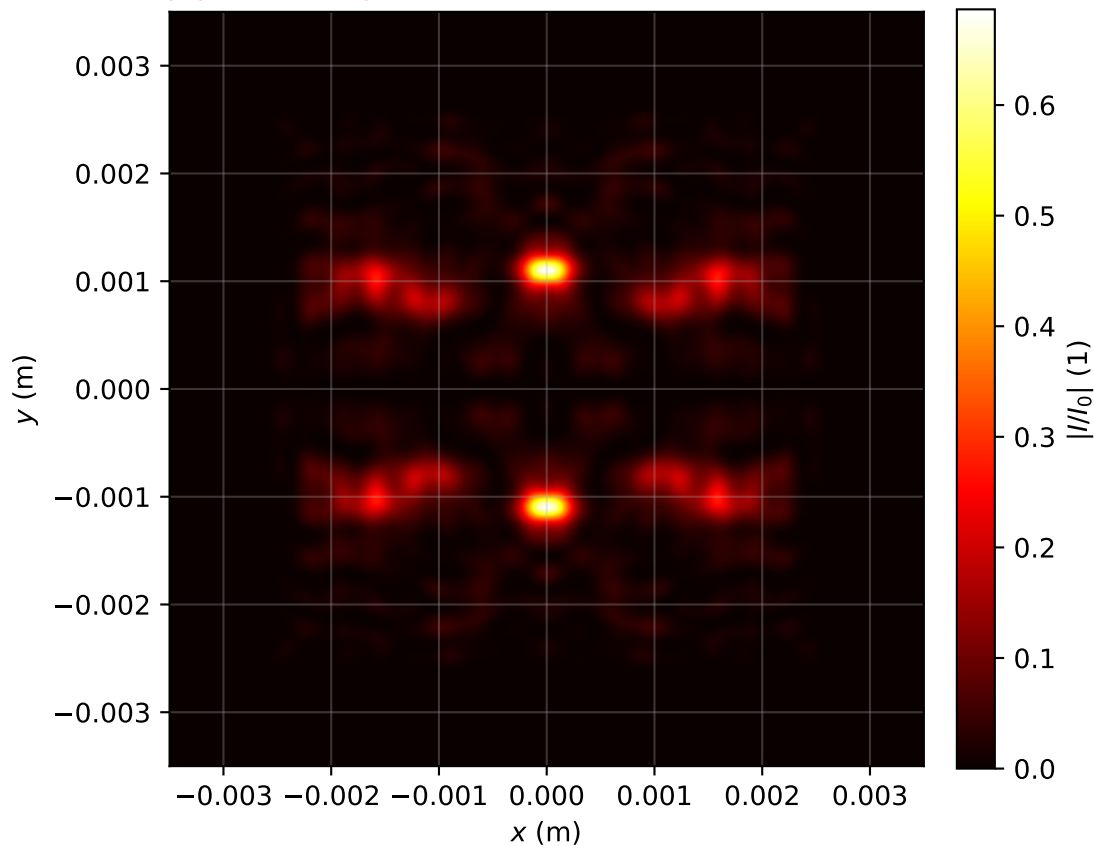
Intensity profile I(x, y, z = 3.184)/I_0 , P_{in}=18.0\text{Pcr} , artificial time
