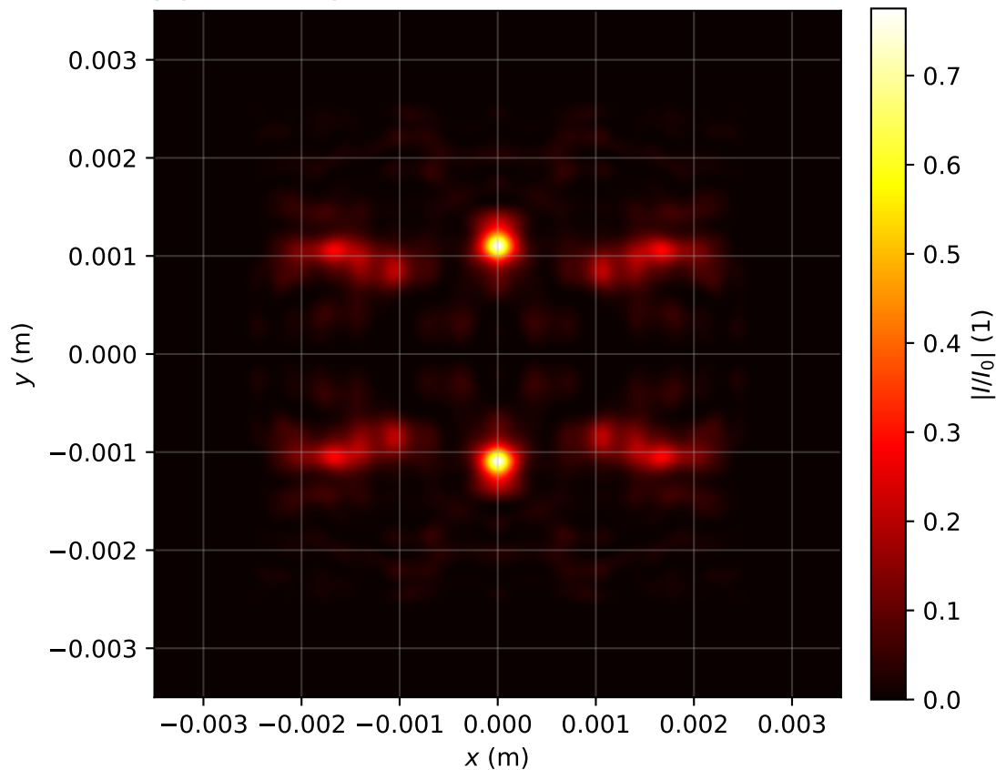
Intensity profile I(x, y, z = 3.264)/I_0 , P_{in}=18.0P_{cr} , artificial time
