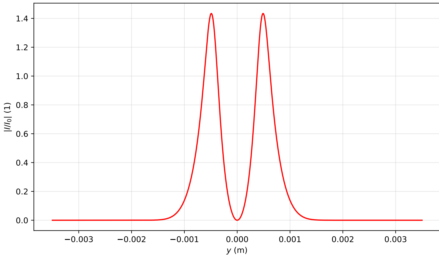
Intensity profile I(x=0, y, z=0.159)/I_0 , P_{in}=18.0\text{Pcr} , artificial time
