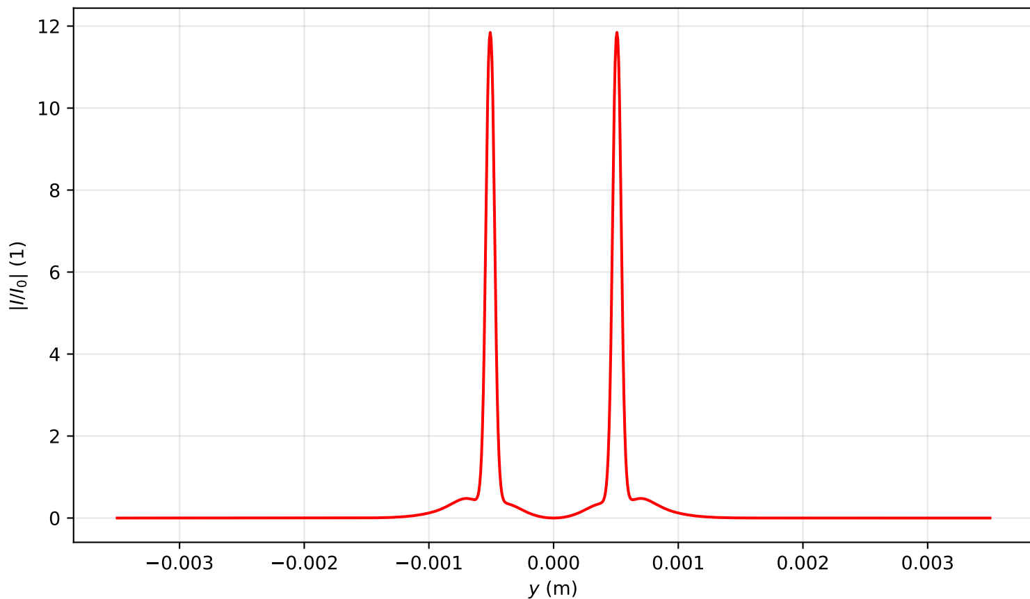
Intensity profile I(x=0, y, z=0.318)/I_0 , Pin=18.0Pcr, artificial time
